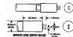
UVB Series - 2 pins each end
