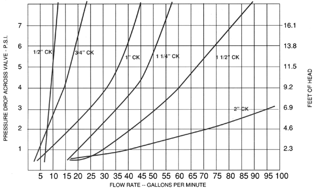
Pressure and Head Loss Check Valve
